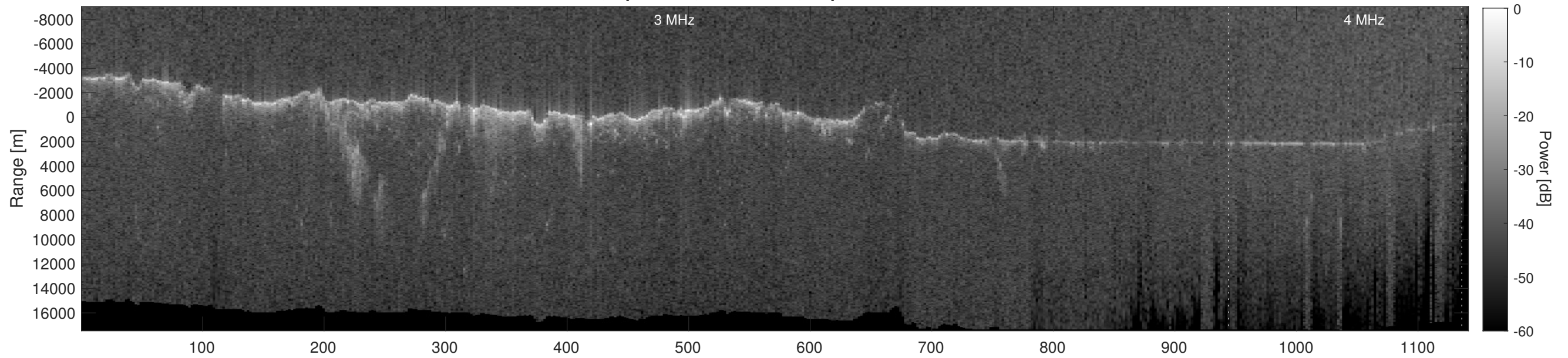
Orbit 10091, Depth-Corrected Cluttergram
