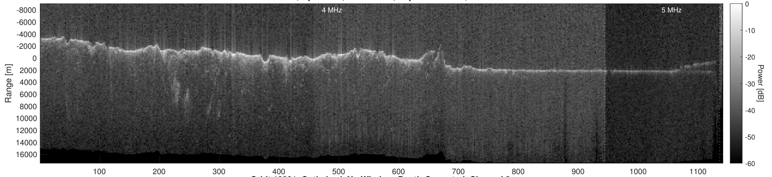
Orbit 10091, Optimized, No Window, Depth-Corrected, Channel 2
