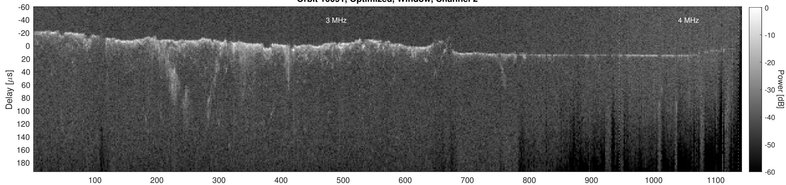
Orbit 10091, Cluttergram
