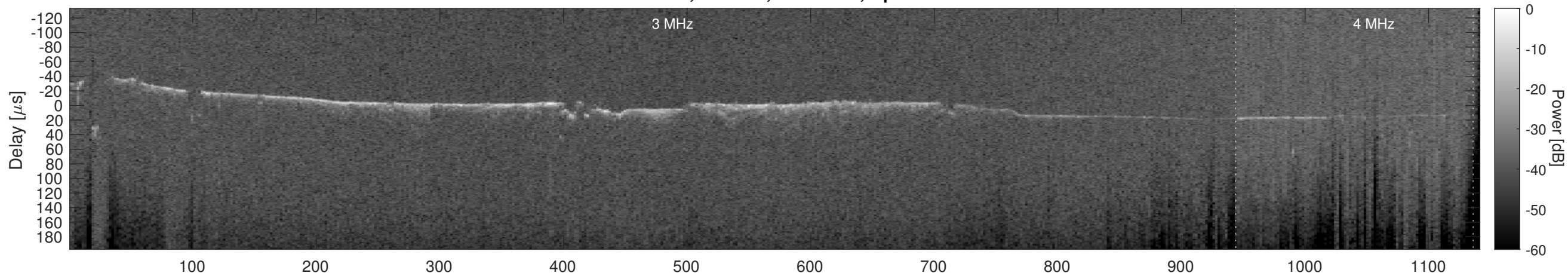
Orbit 10092, Cluttergram
