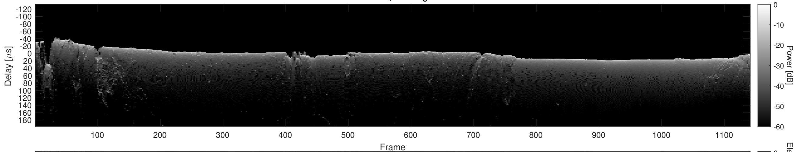
Orbit 10092, Cluttergram
