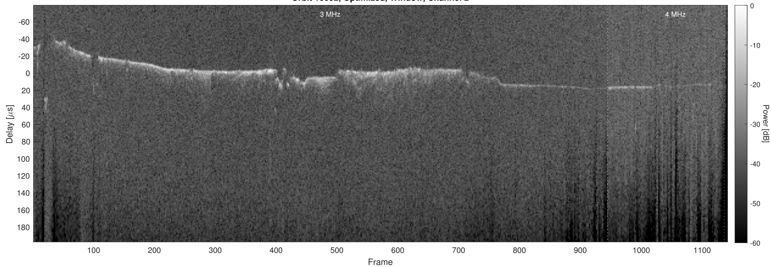
Orbit 10092, Optimized, Window, Channel 2
