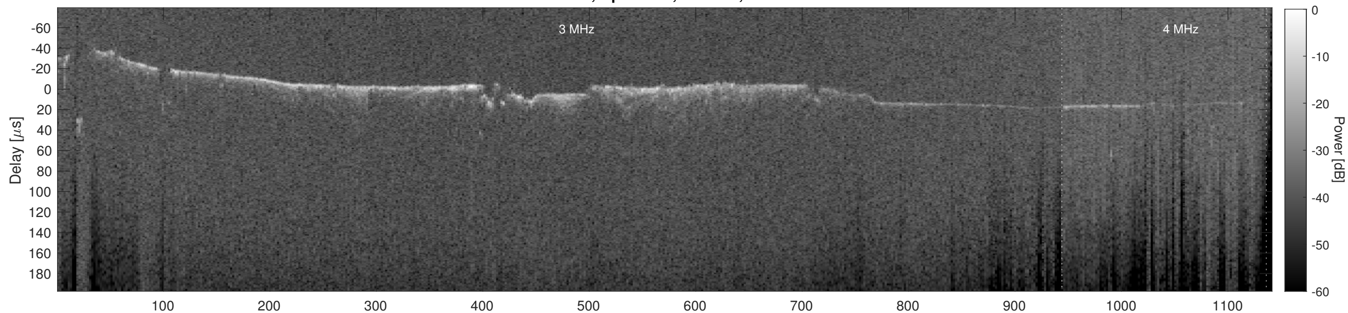
Orbit 10092, Cluttergram
