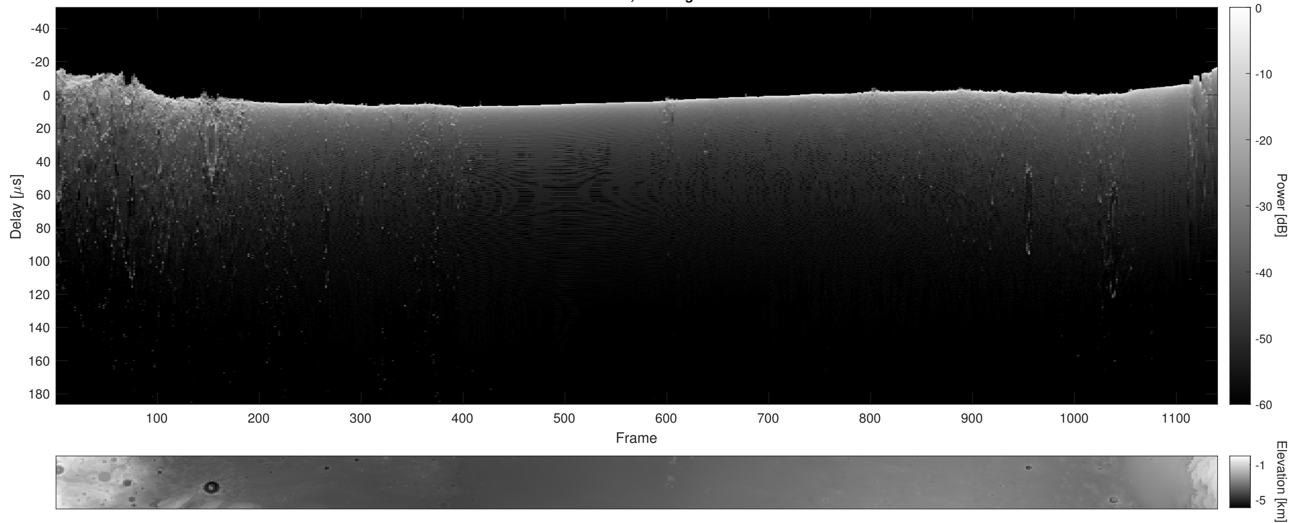
Orbit 10093, Cluttergram
