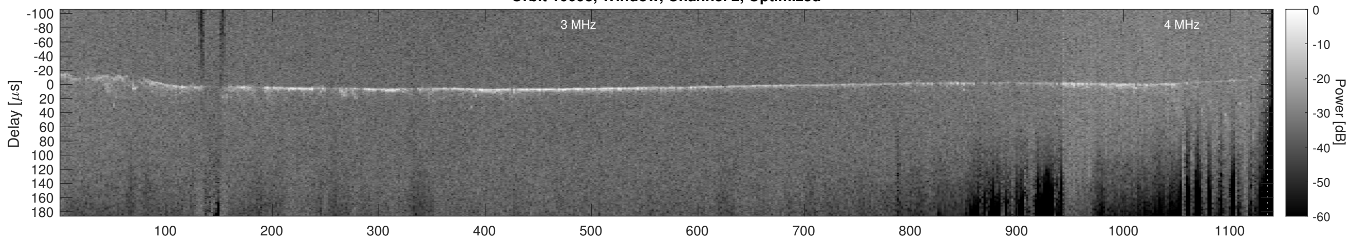
Orbit 10093, Cluttergram
