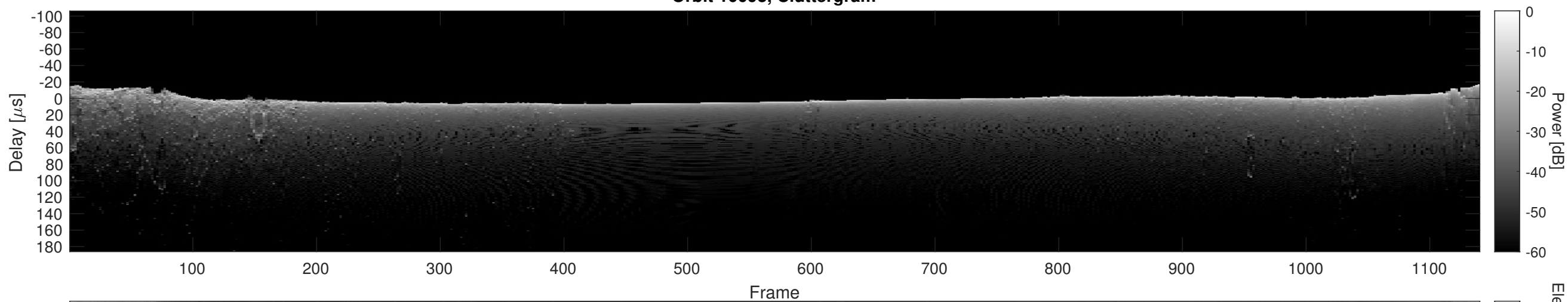
Orbit 10093, Cluttergram
