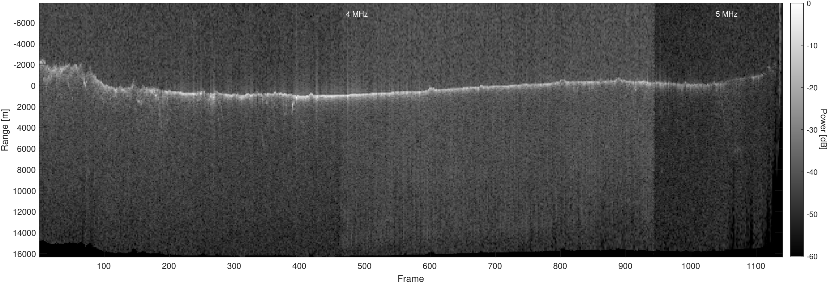
Orbit 10093, Optimized, No Window, Depth-Corrected, Channel 2
