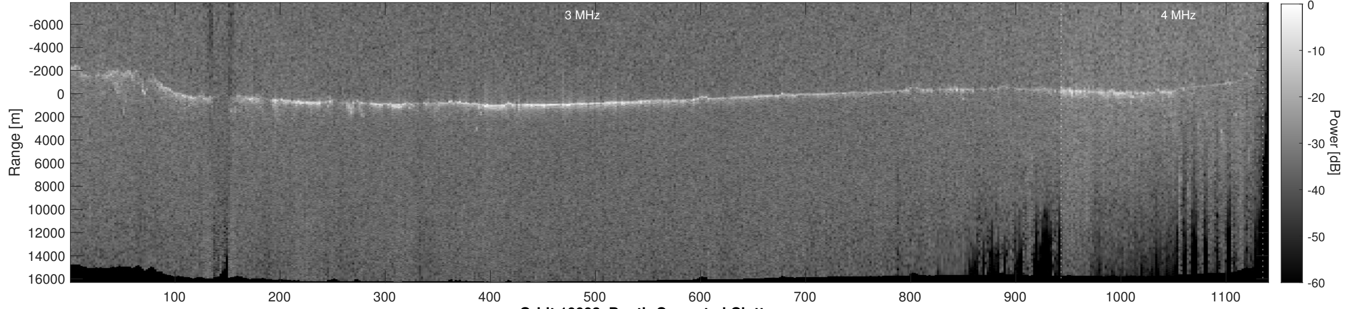
Orbit 10093, Depth-Corrected Cluttergram
