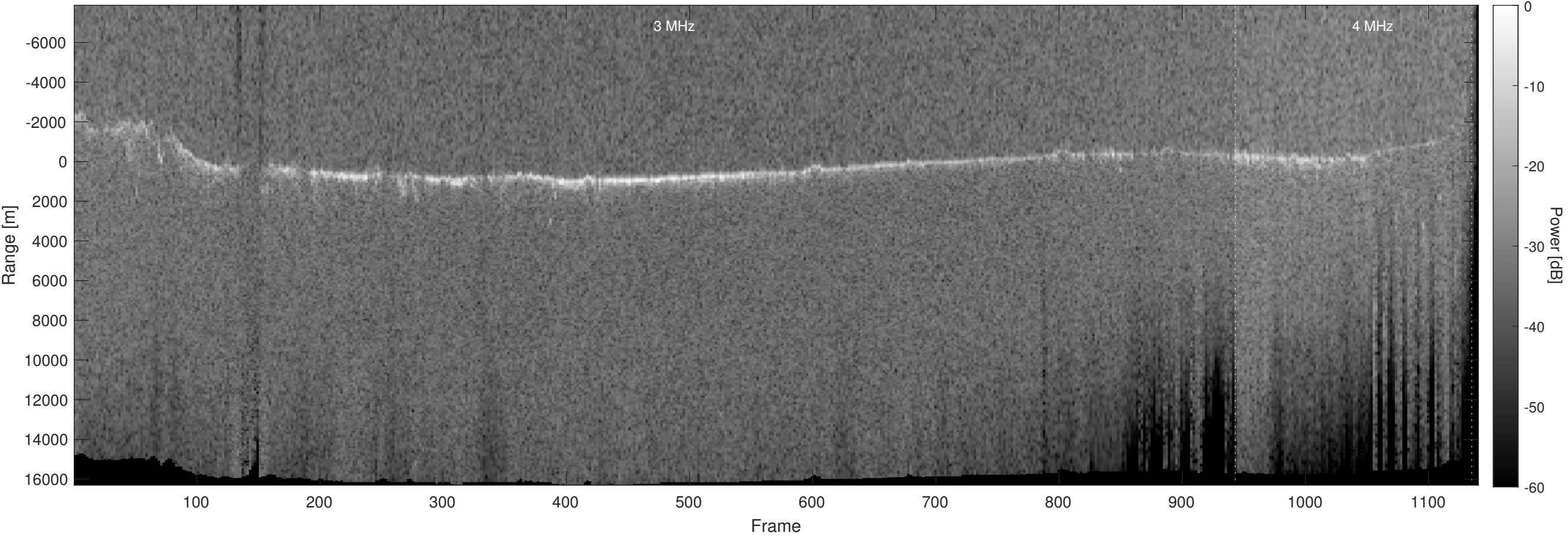
Orbit 10093, Optimized, Window, Depth-Corrected, Channel 2
