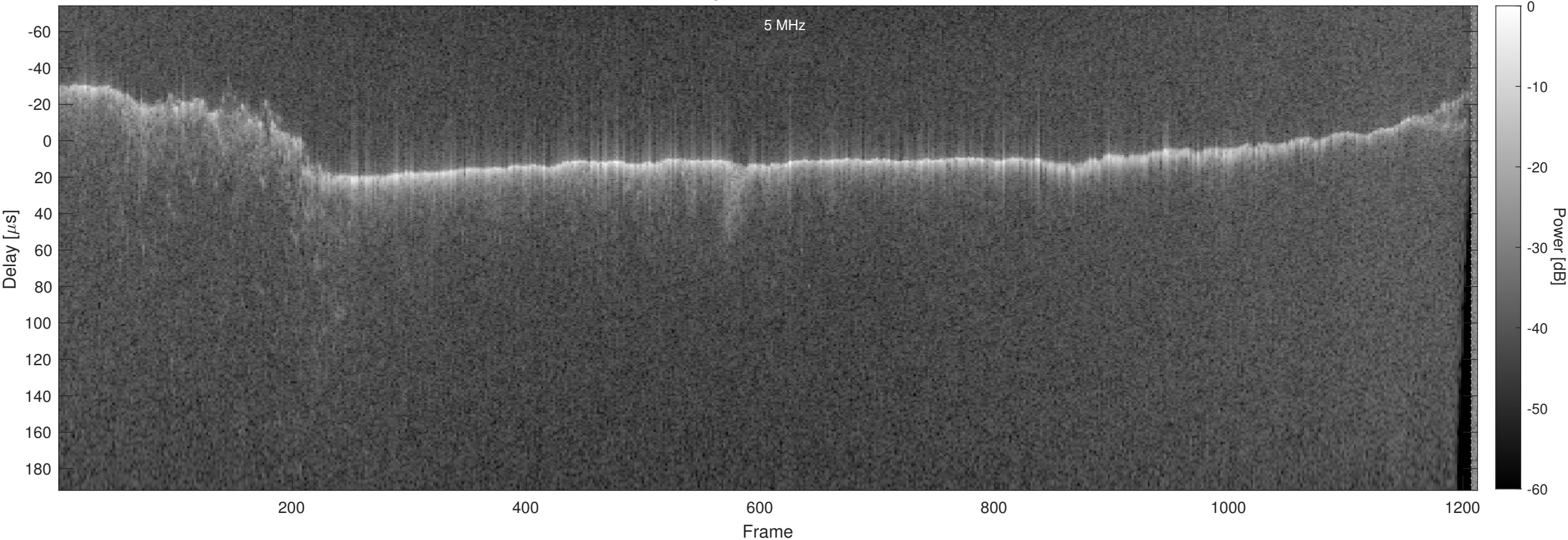
Orbit 10094, Chapman, No Window, Channel 2
