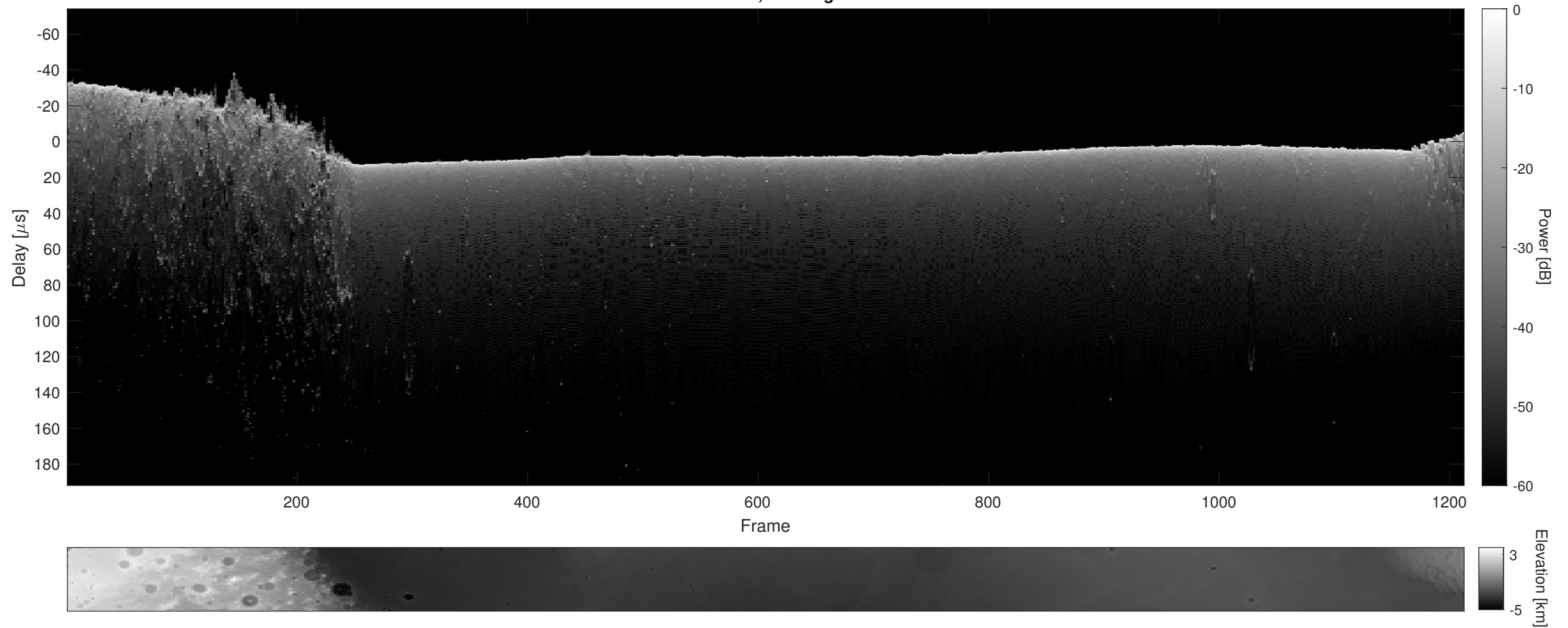
Orbit 10094, Cluttergram
