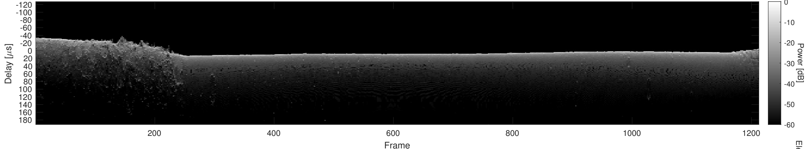
Orbit 10094, Cluttergram
