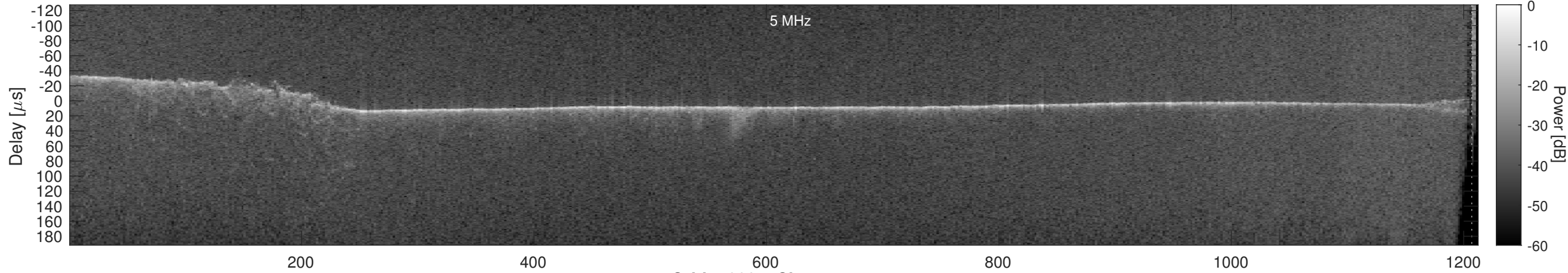
Orbit 10094, Cluttergram
