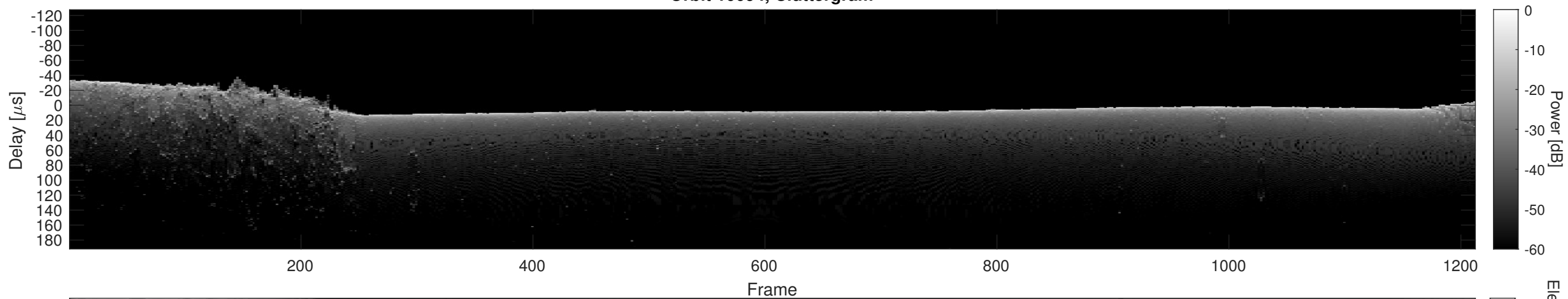
Orbit 10094, Cluttergram
