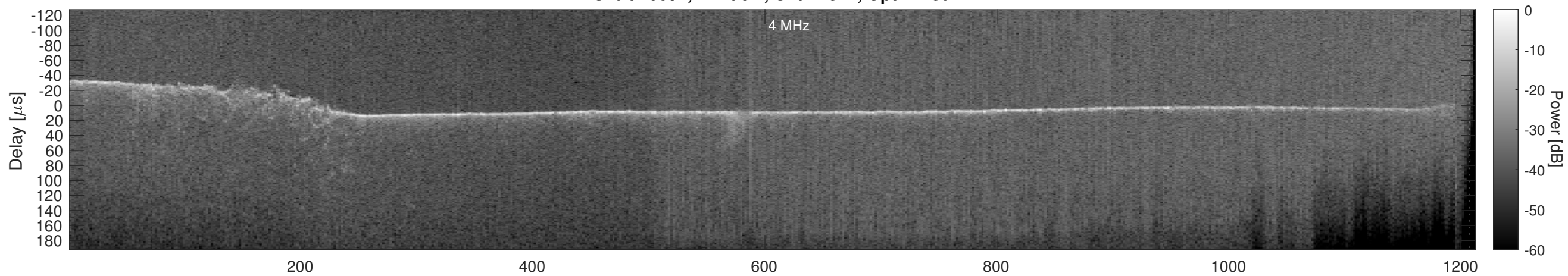
Orbit 10094, Cluttergram
