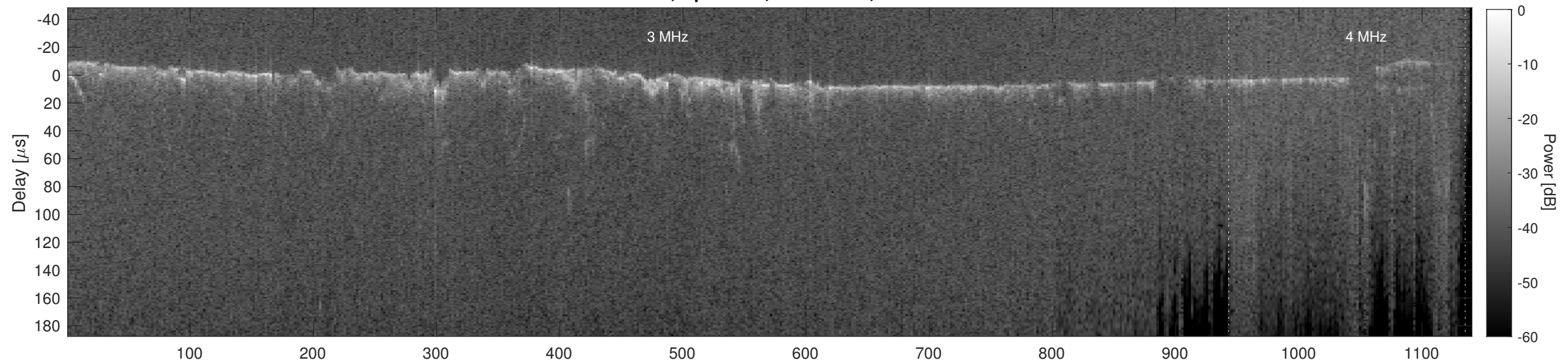
Orbit 10095, Cluttergram
