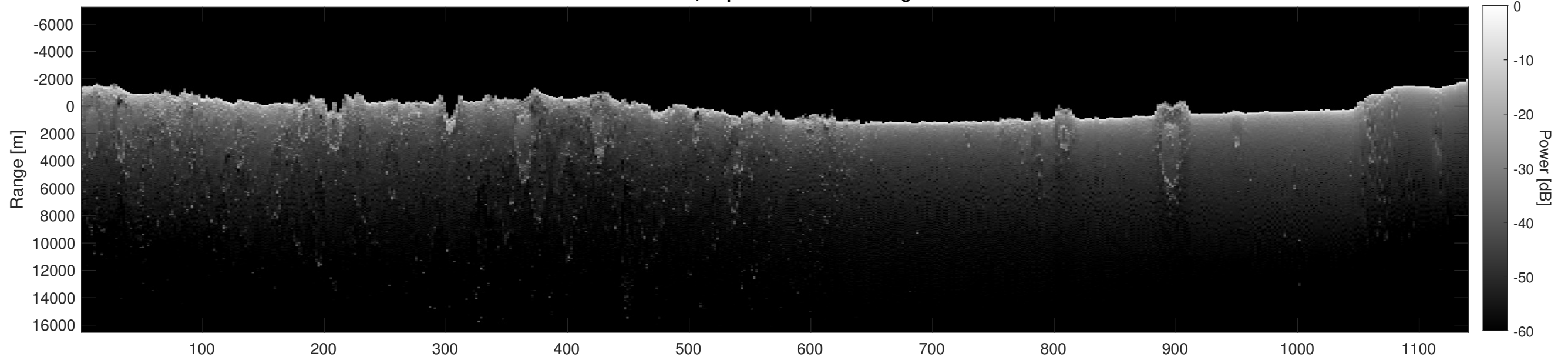
Orbit 10095, Depth-Corrected Cluttergram
