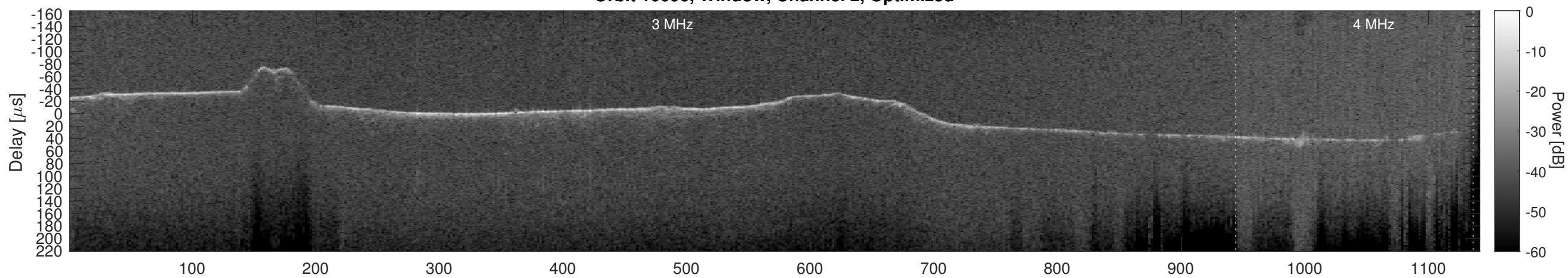
Orbit 10096, Cluttergram
