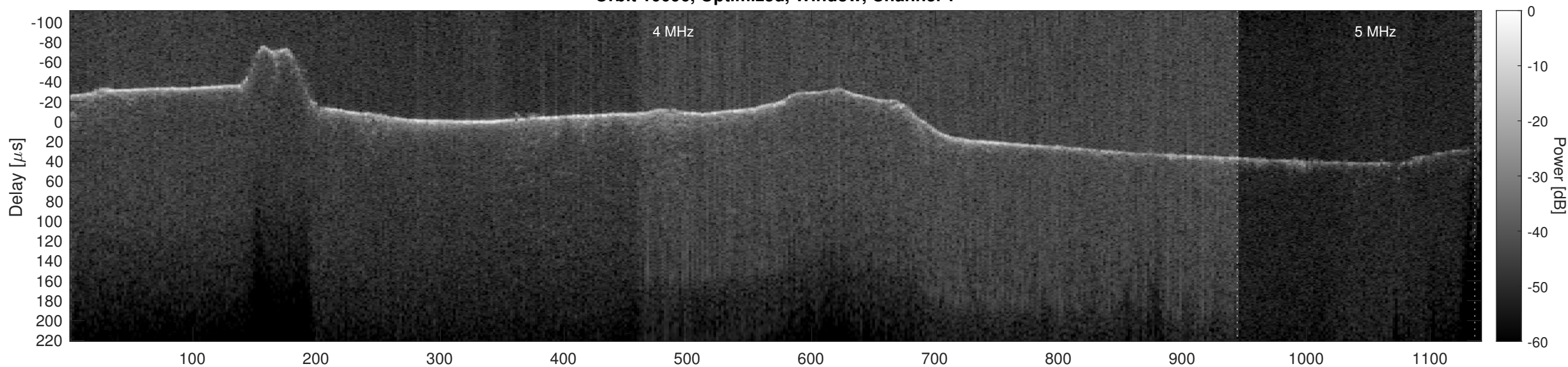
Orbit 10096, Optimized, Window, Channel 2
