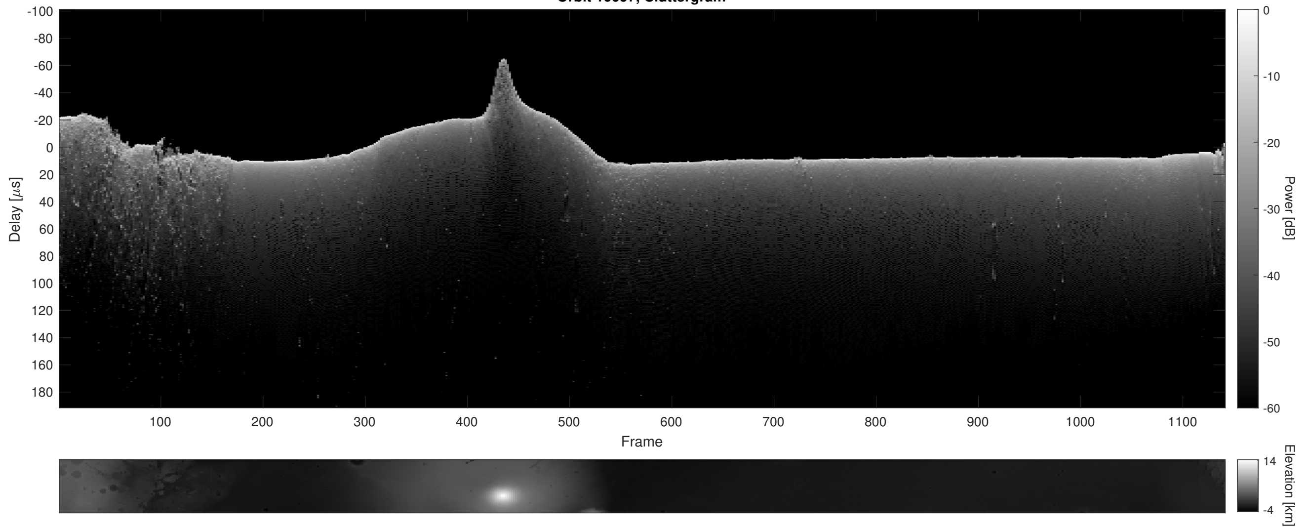
Orbit 10097, Cluttergram
