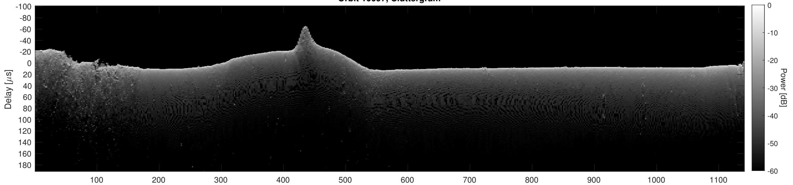
Orbit 10097, Cluttergram
