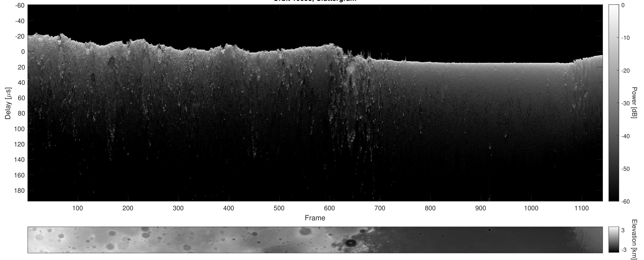
Orbit 10098, Cluttergram
