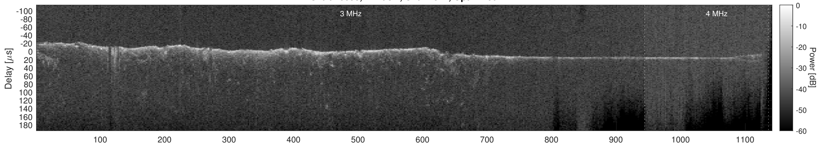
Orbit 10098, Cluttergram
