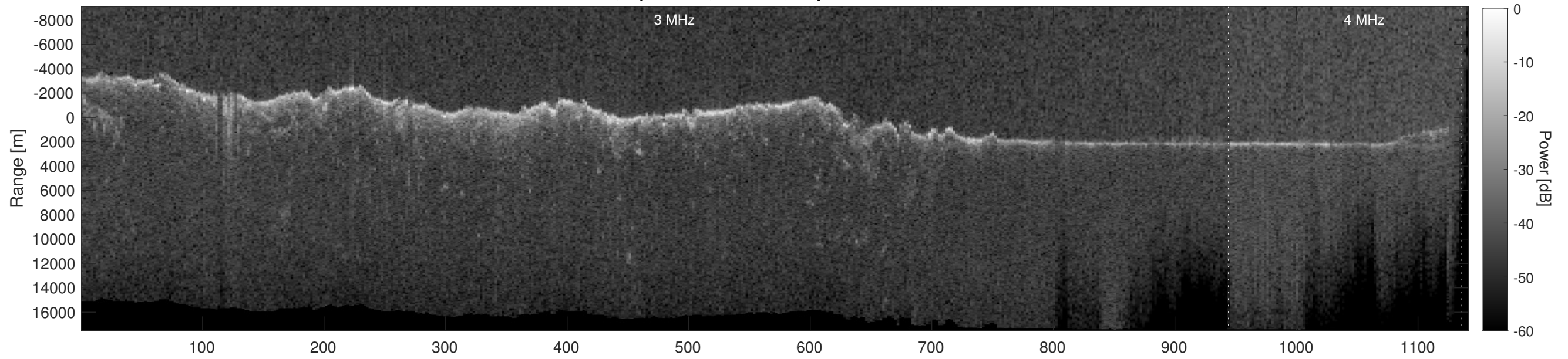
Orbit 10098, Depth-Corrected Cluttergram
