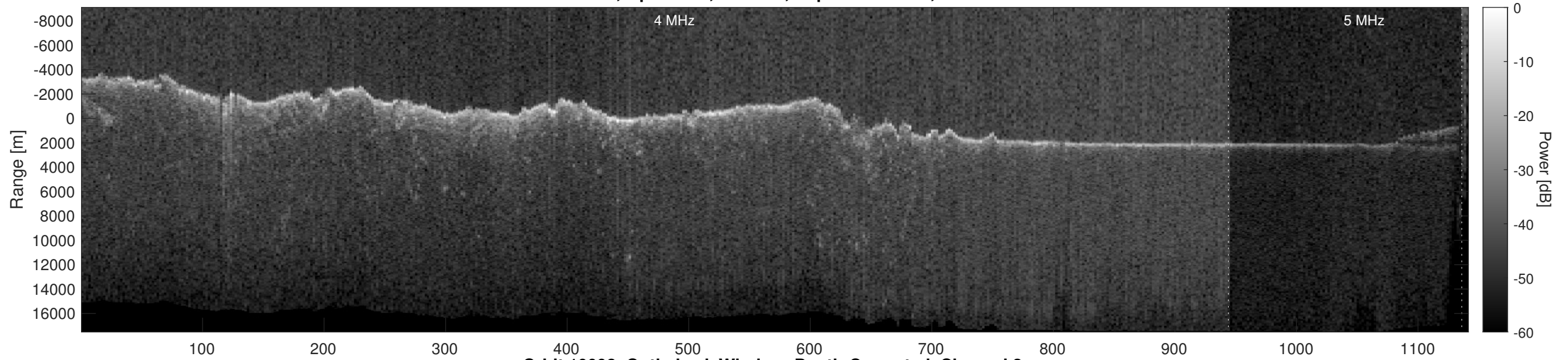
Orbit 10098, Optimized, Window, Depth-Corrected, Channel 2
