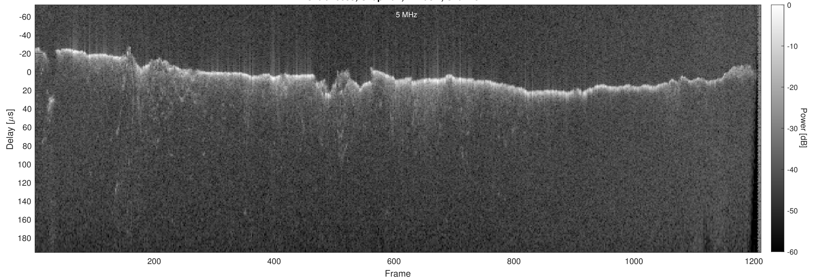
Orbit 10099, Chapman, Window, Channel 2
