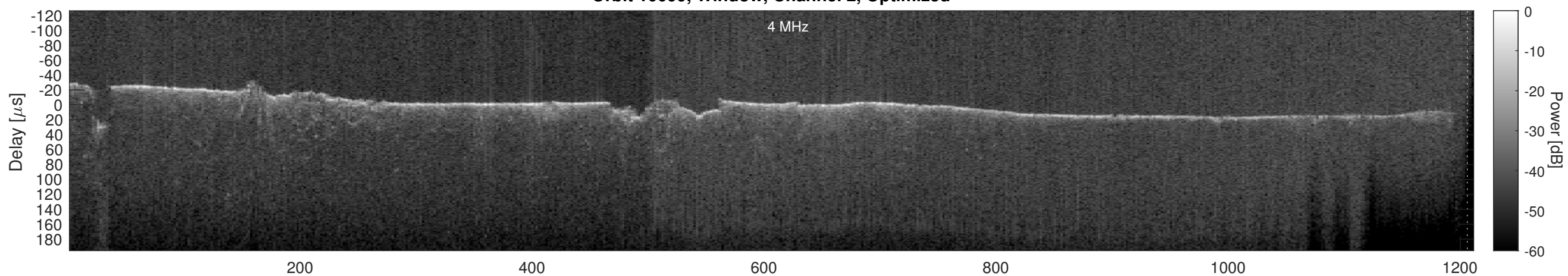
Orbit 10099, Cluttergram
