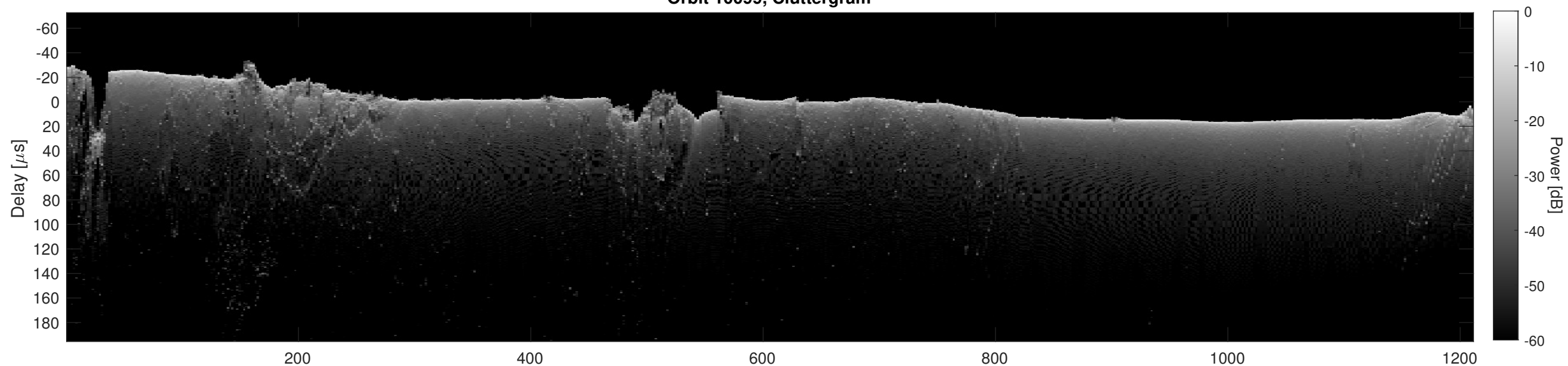
Orbit 10099, Cluttergram
