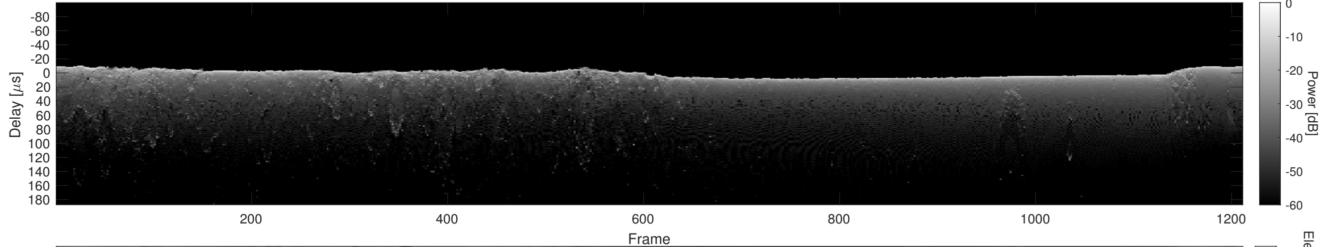
Orbit 10102, Cluttergram
