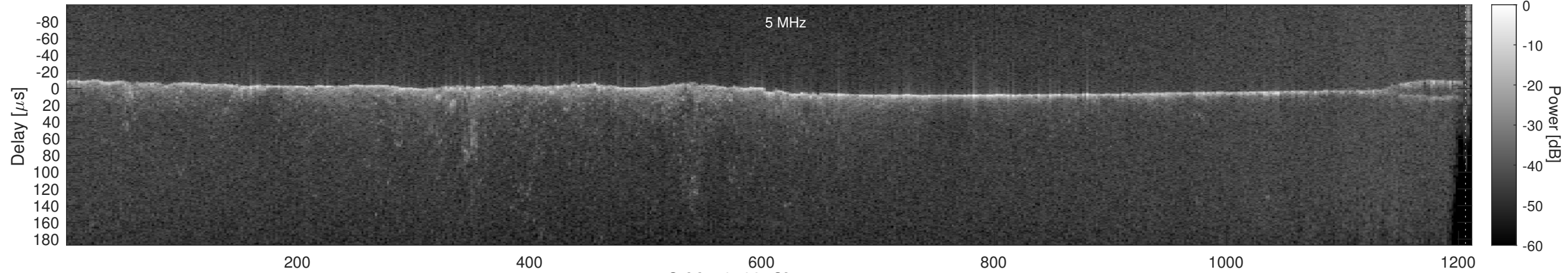
Orbit 10102, Cluttergram
