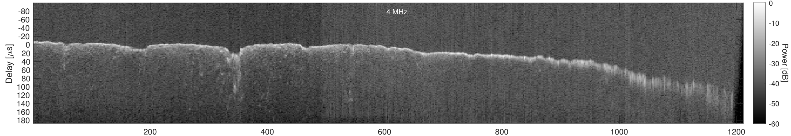
Orbit 10102, Window, Channel 2, Chapman
