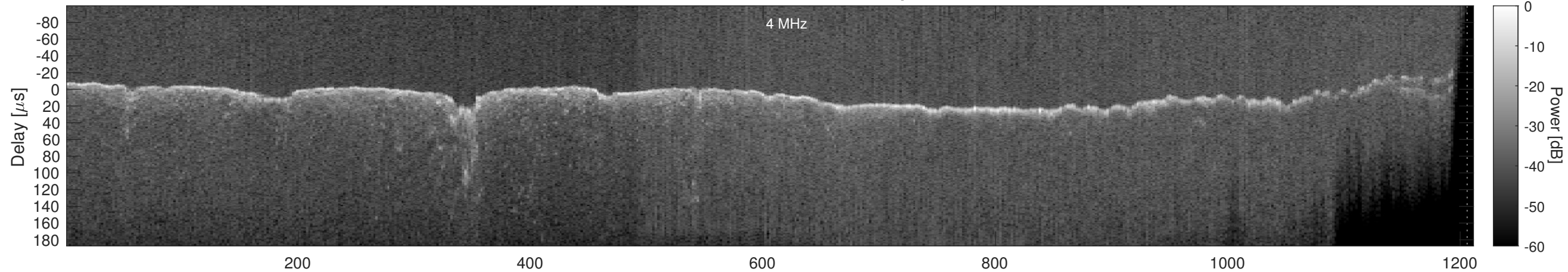
Orbit 10102, Window, Channel 2, Optimized
