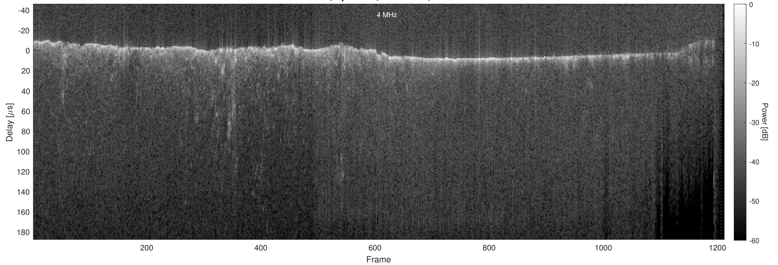
Orbit 10102, Optimized, No Window, Channel 2
