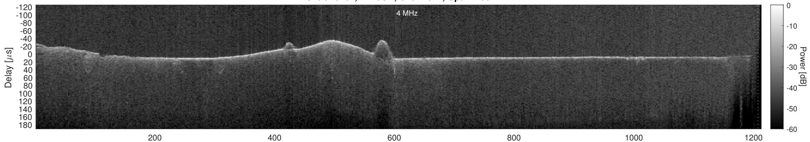
Orbit 10104, Cluttergram
