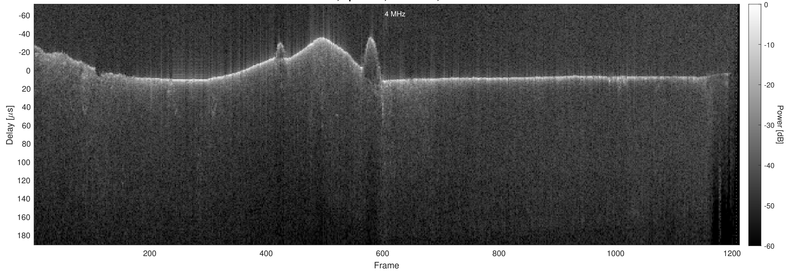
Orbit 10104, Optimized, No Window, Channel 2
