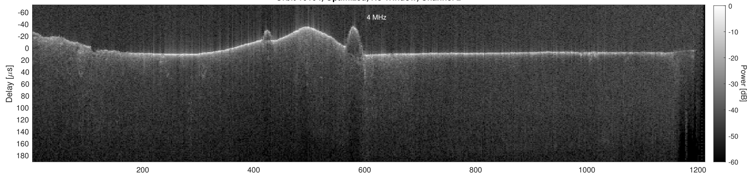
Orbit 10104, Cluttergram
