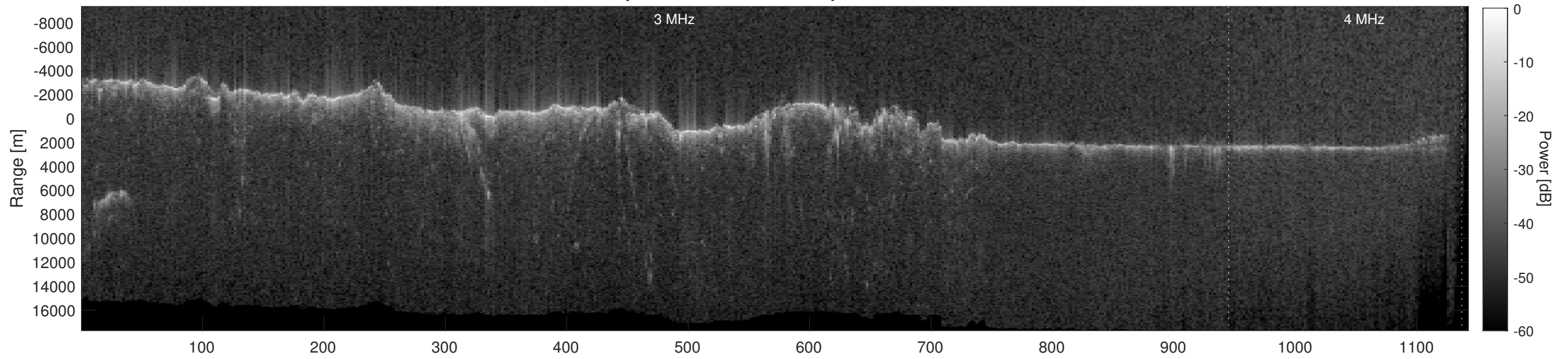
Orbit 10105, Depth-Corrected Cluttergram
