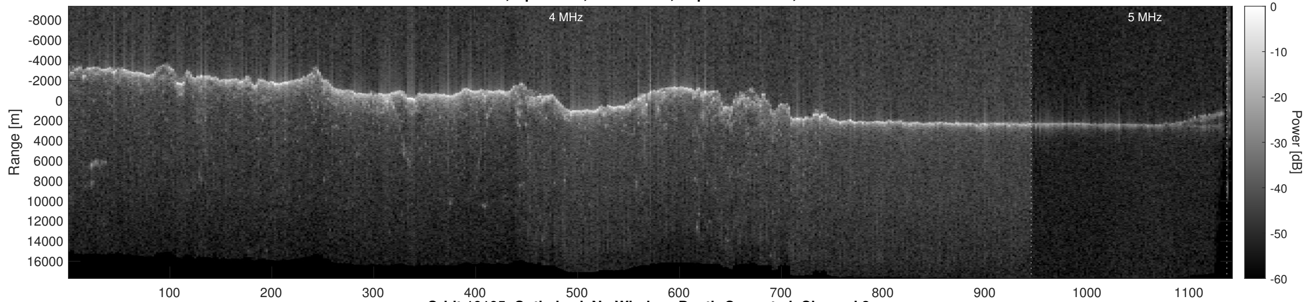
Orbit 10105, Optimized, No Window, Depth-Corrected, Channel 2
