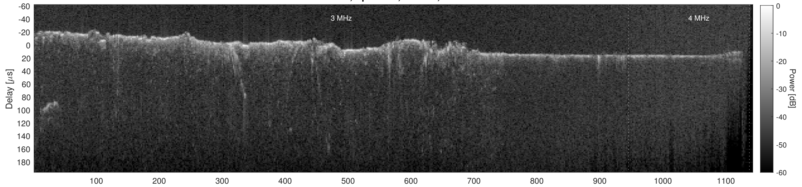
Orbit 10105, Cluttergram
