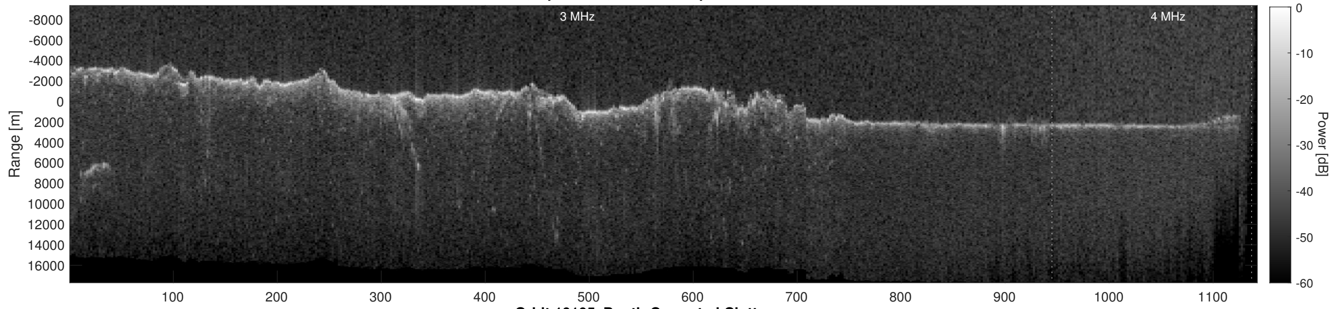
Orbit 10105, Depth-Corrected Cluttergram
