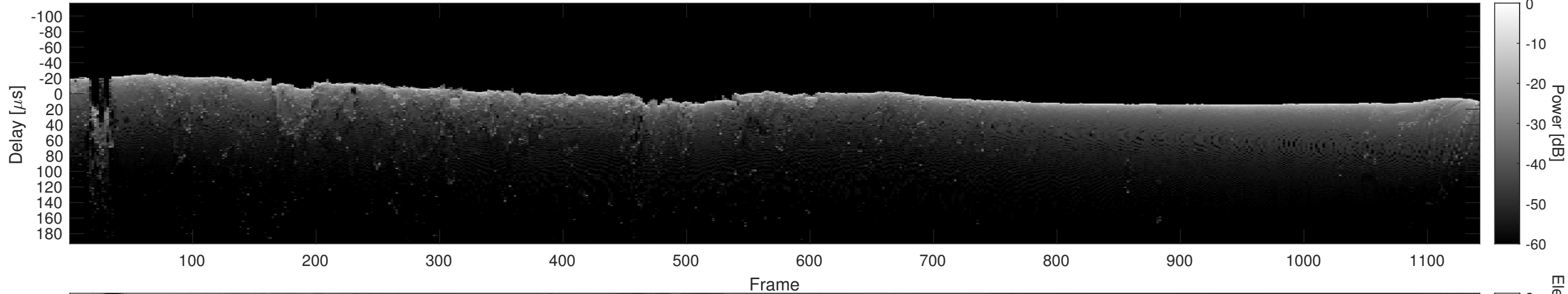
Orbit 10106, Cluttergram
