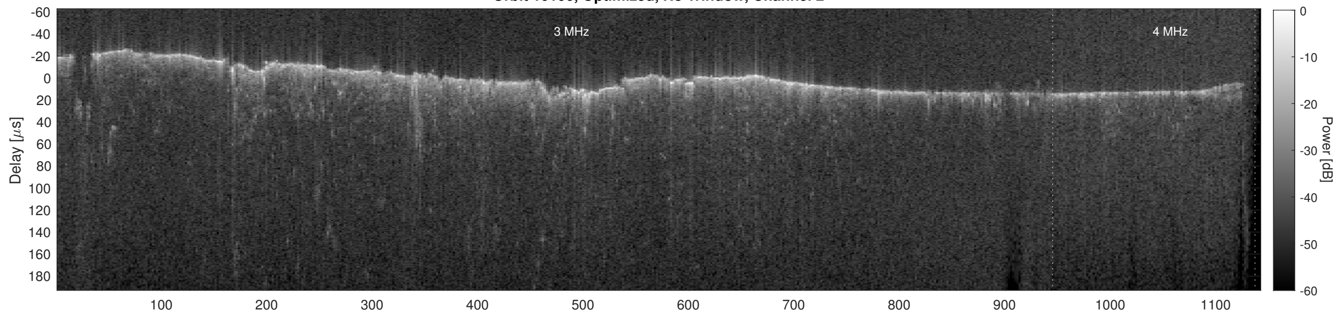
Orbit 10106, Cluttergram
