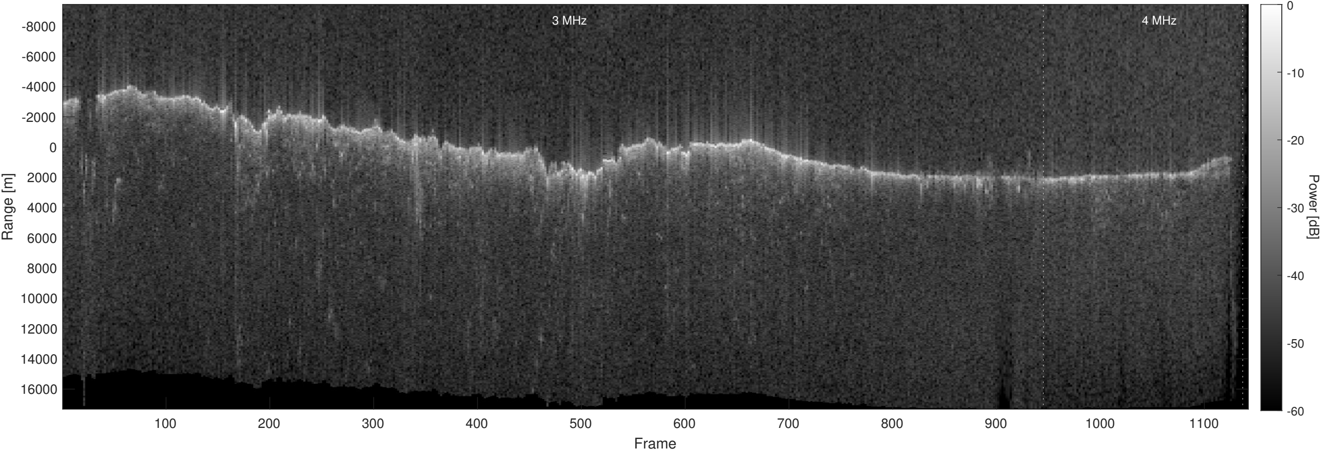
Orbit 10106, Optimized, No Window, Depth-Corrected, Channel 2
