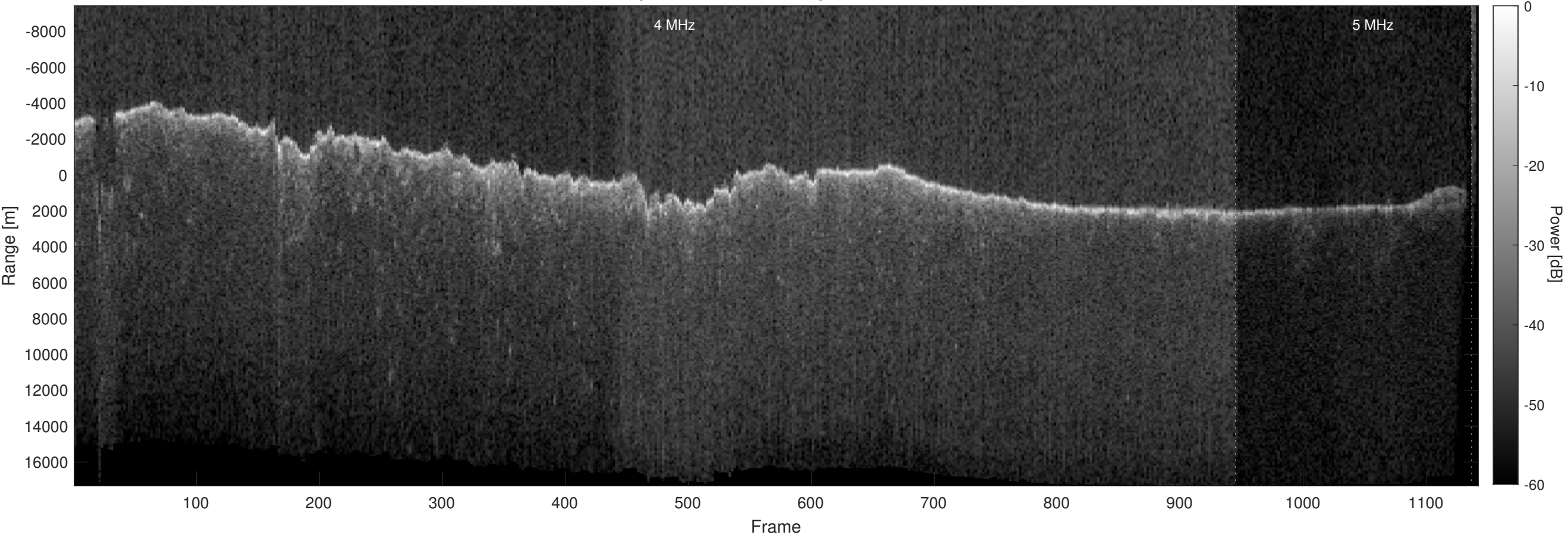
Orbit 10106, Optimized, Window, Depth-Corrected, Channel 2
