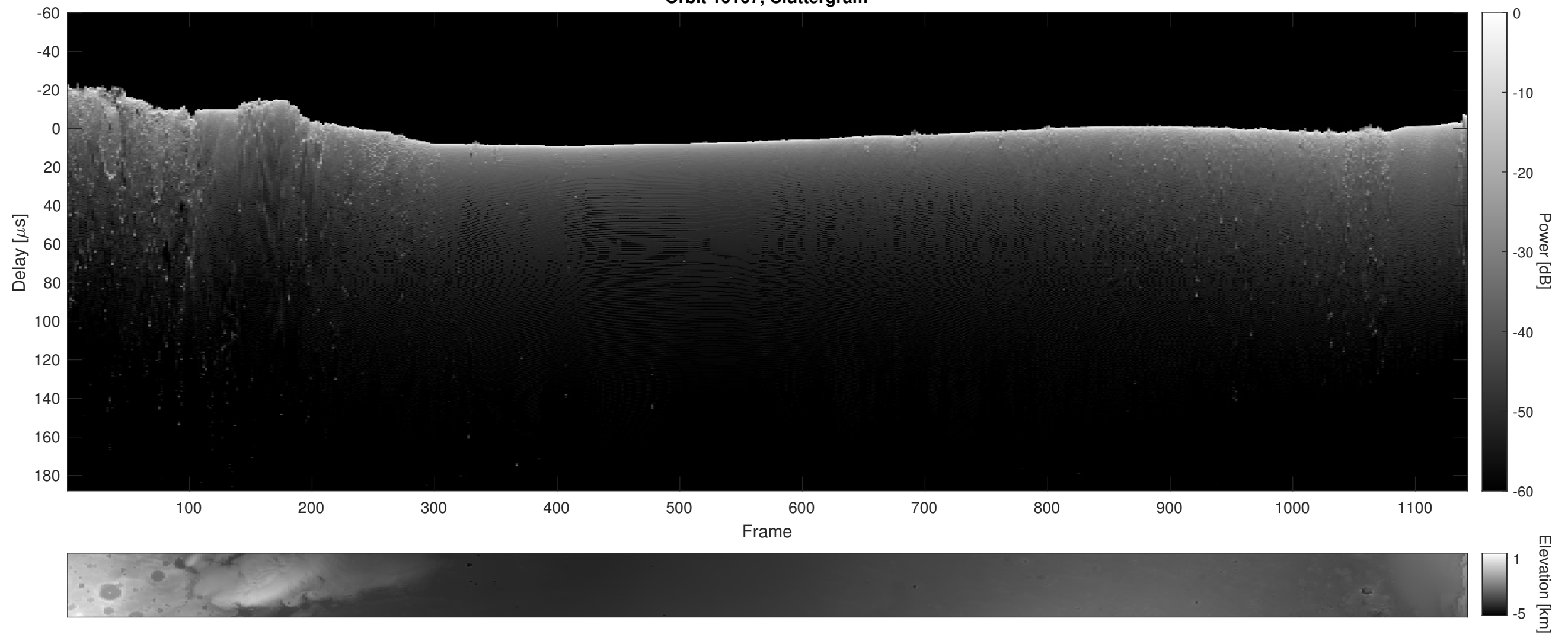
Orbit 10107, Cluttergram
