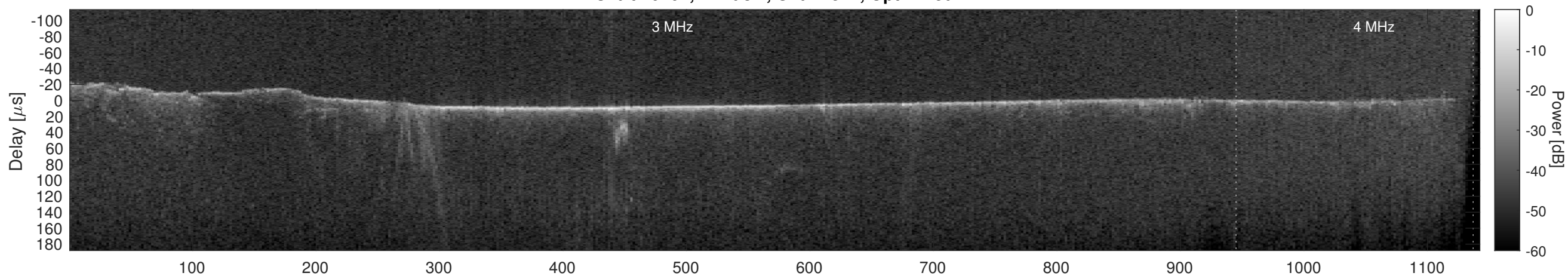
Orbit 10107, Cluttergram
