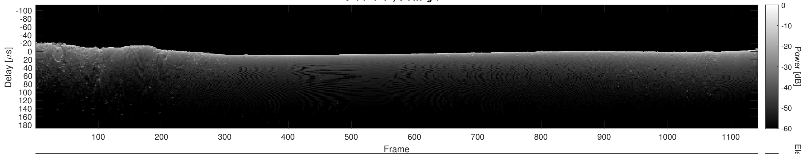
Orbit 10107, Cluttergram
