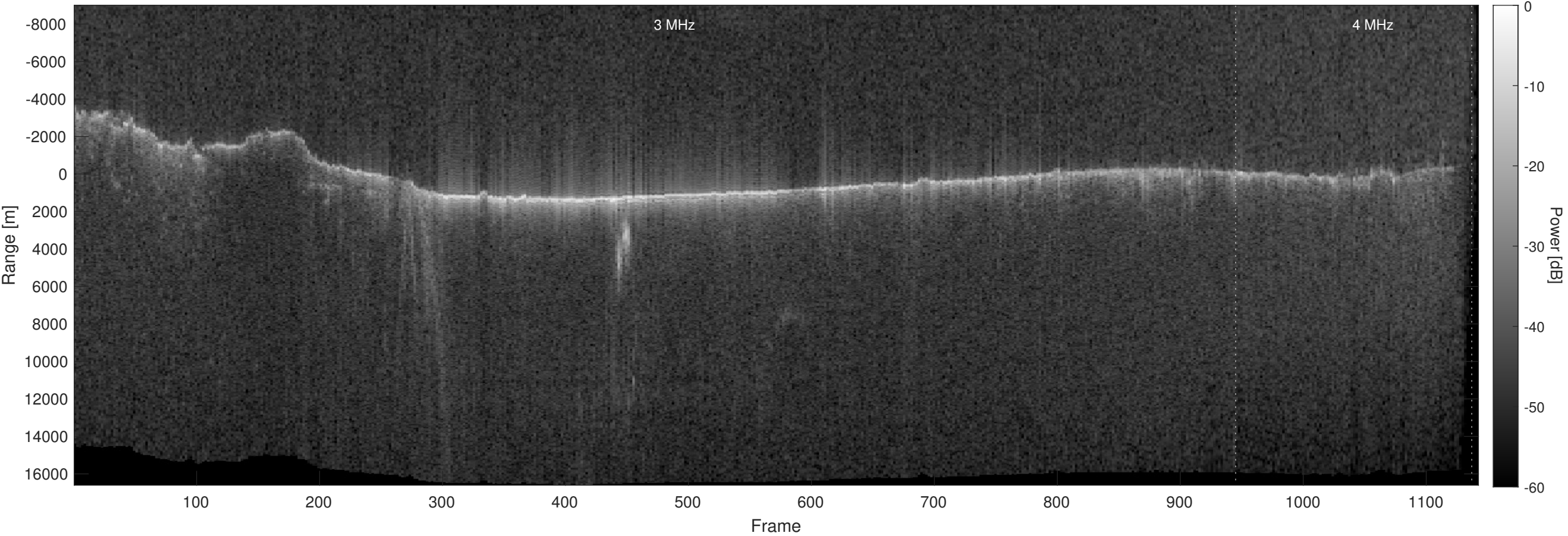
Orbit 10107, Optimized, No Window, Depth-Corrected, Channel 2
