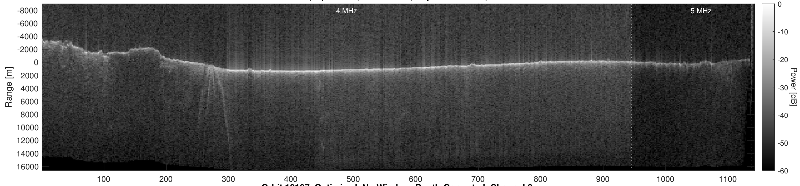
Orbit 10107, Optimized, No Window, Depth-Corrected, Channel 2
