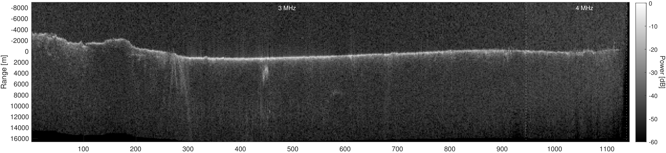
Orbit 10107, Depth-Corrected Cluttergram
