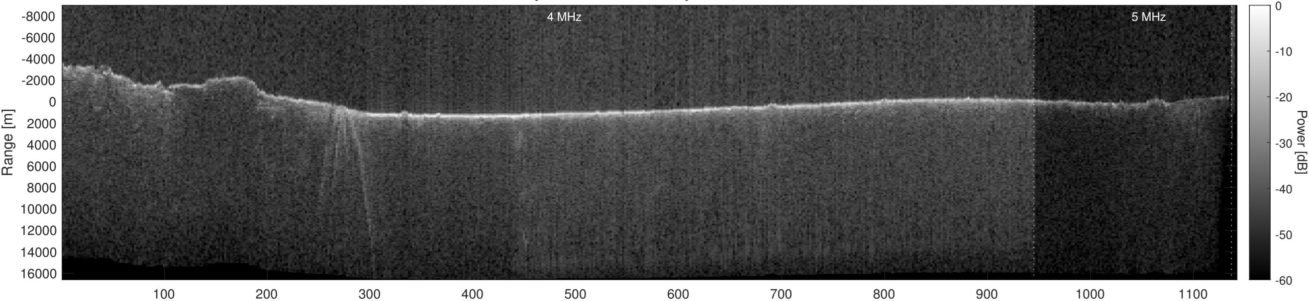
Orbit 10107, Optimized, Window, Depth-Corrected, Channel 2
