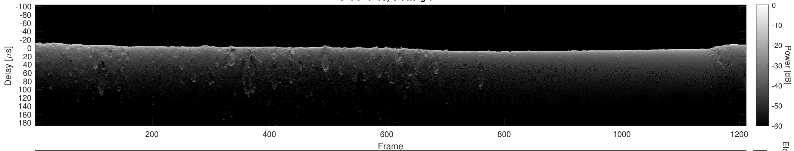
Orbit 10109, Cluttergram
