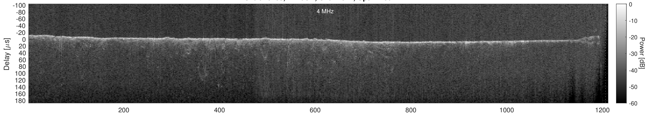
Orbit 10109, Cluttergram
