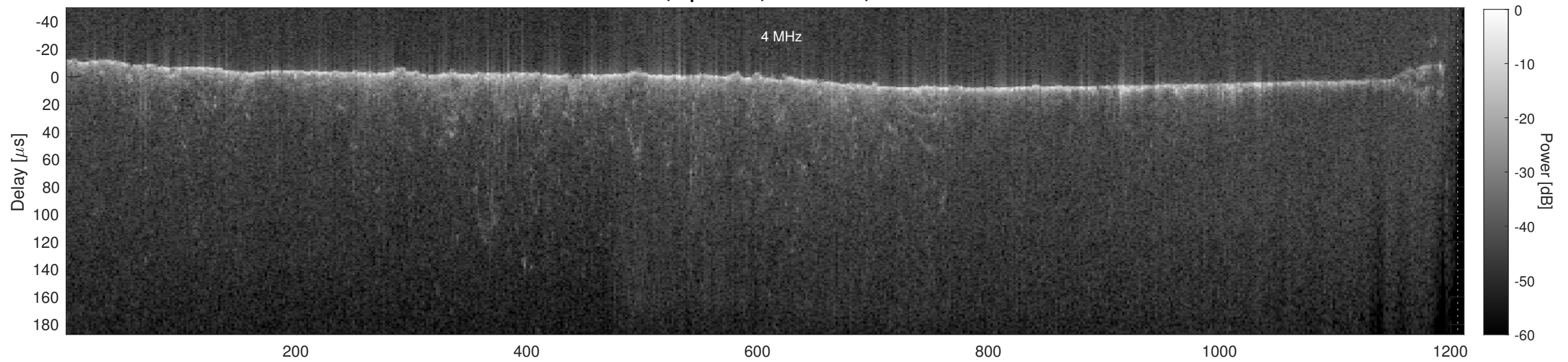
Orbit 10109, Cluttergram
