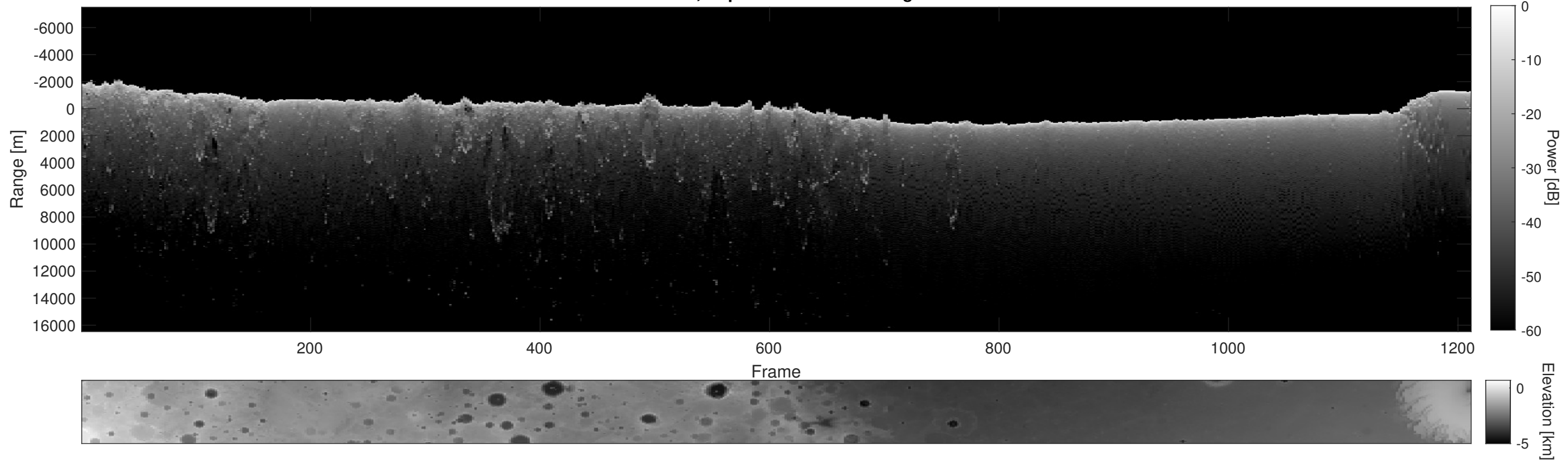
Orbit 10109, Depth-Corrected Cluttergram
