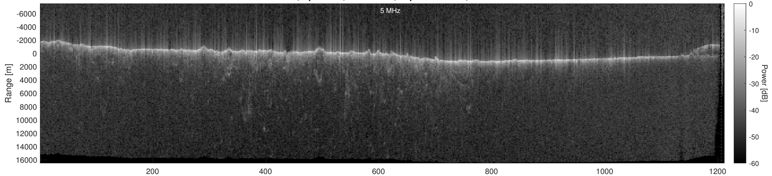
Orbit 10109, Optimized, No Window, Depth-Corrected, Channel 2
