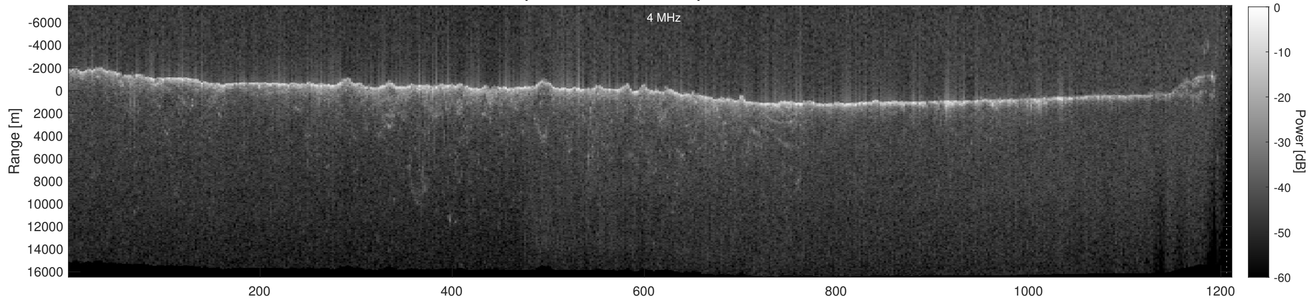
Orbit 10109, Depth-Corrected Cluttergram
