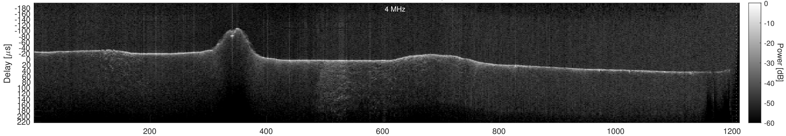
Orbit 10110, Cluttergram
