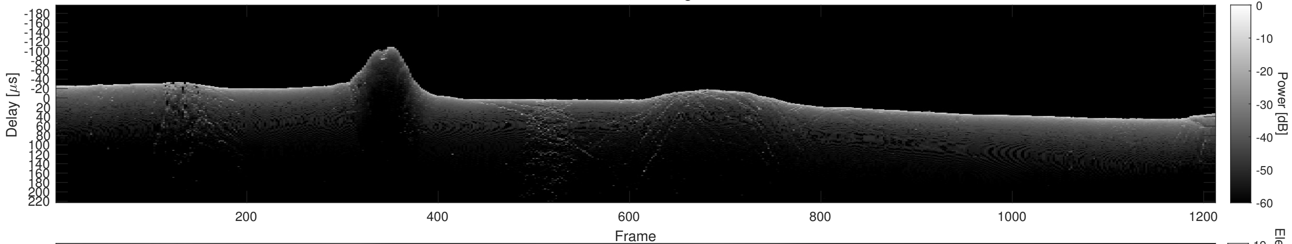
Orbit 10110, Cluttergram
