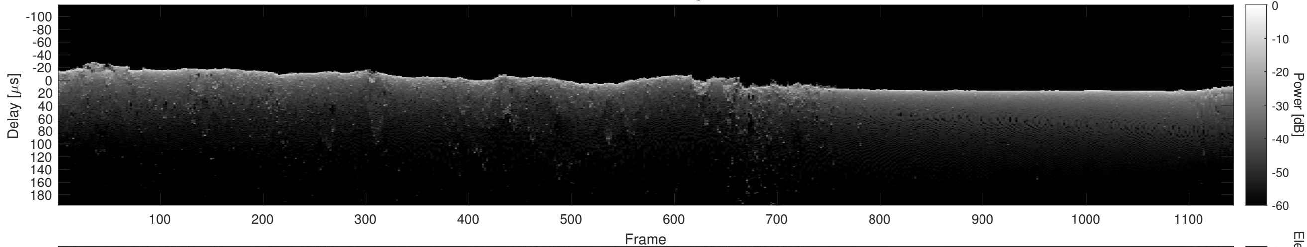
Orbit 10112, Cluttergram
