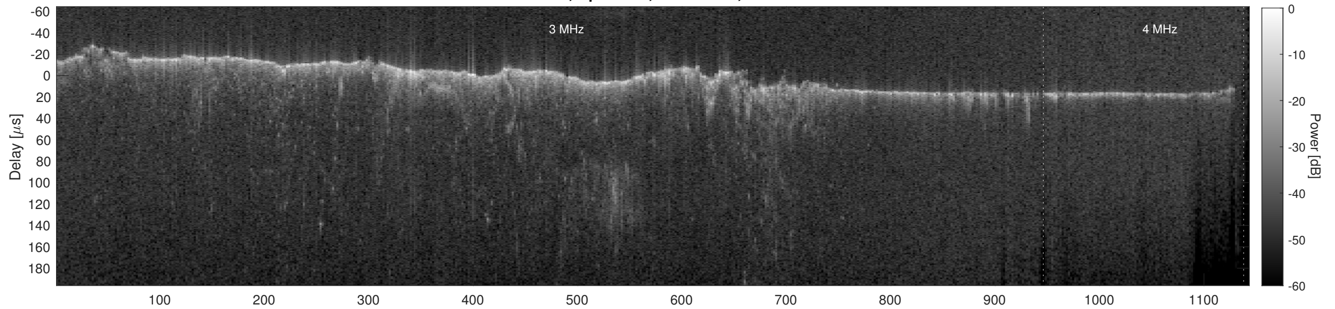
Orbit 10112, Cluttergram
